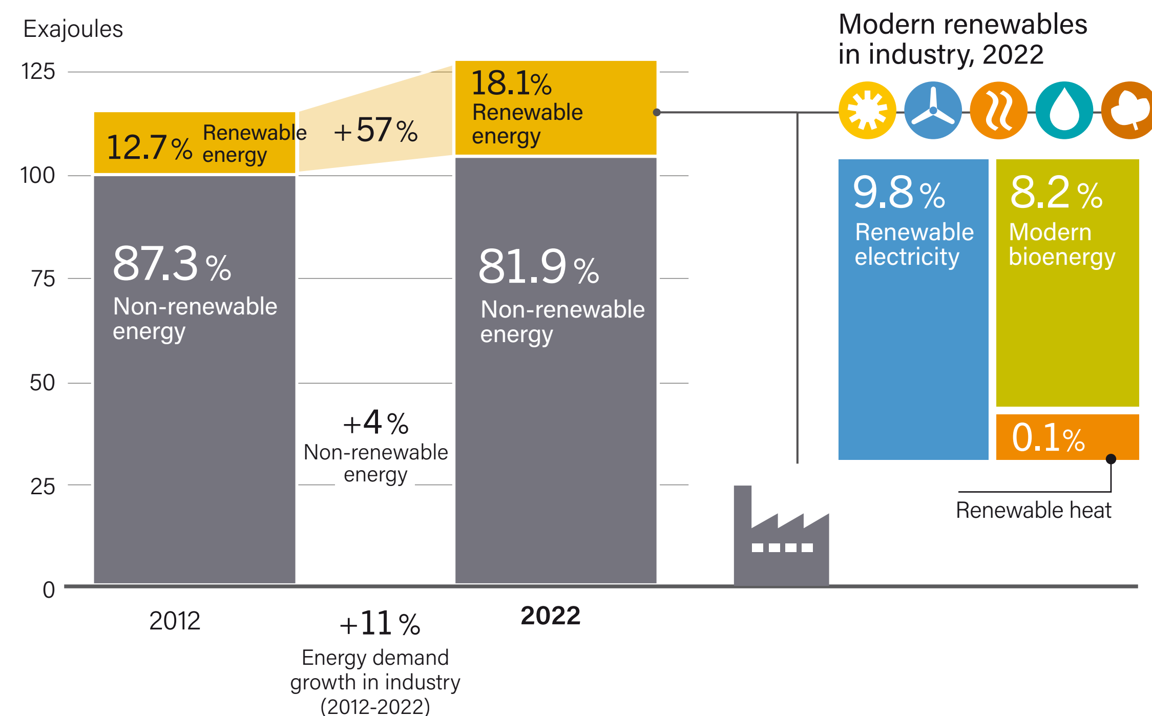
FIGURE I-1 Renewable Share of Total Final Energy Consumption in Industry, 2012 and 2022
